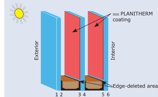
Insulating glass unit with SGG PLANITHERM (coating on faces 3 and 5)
